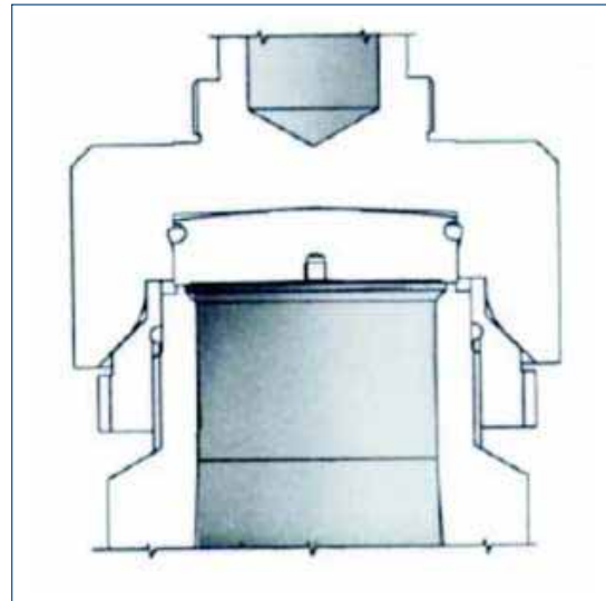
Special trim for liquids(series 100-SV/LIQ)
