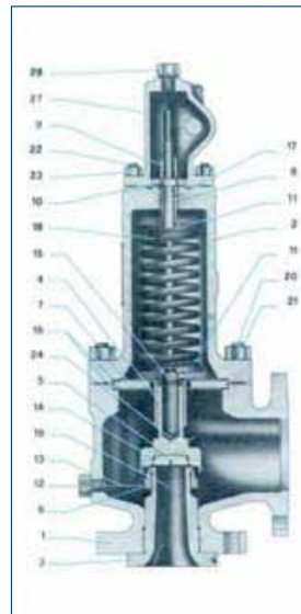
Conventional Valve
