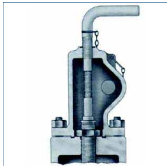
Cap with test gag
