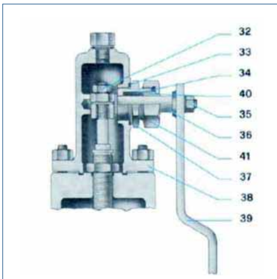
Cap with packed or plain lever
