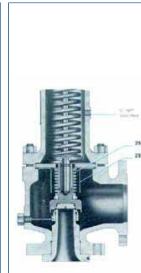
Bellows Valve
